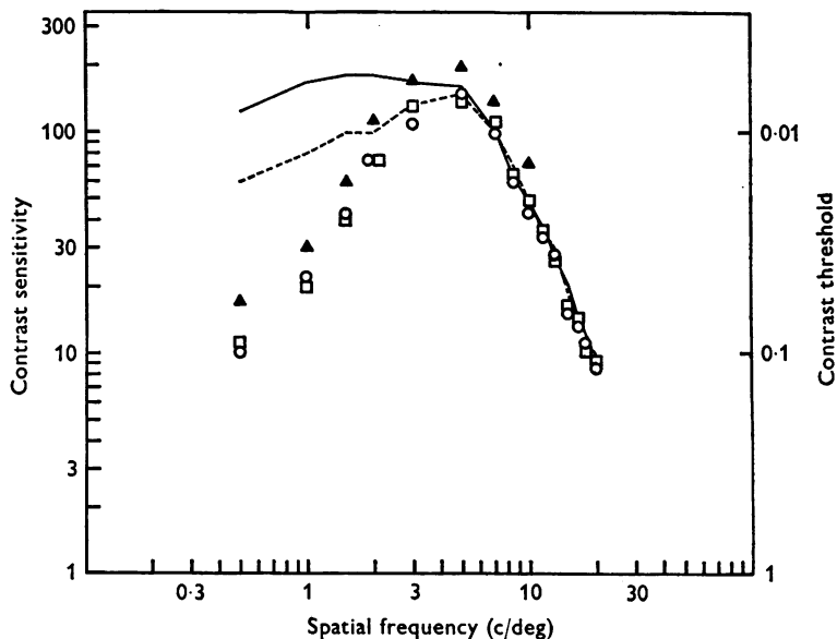
Fig. 3. The sensitivity for pattern recognition as a function of spatial frequency. The gratings were either alternated in phase at 3.5 Hz (○) or were switched on and off at the same rate (□). The continuous and interrupted lines show the sensitivities for detecting the stimulus irrespective of its appearance, reproduced from Fig. 1. The filled triangles show the sensitivity for detecting stationary sinusoidal gratings. Mean luminance 7 cd/m 2 . Subject J.J.K.
